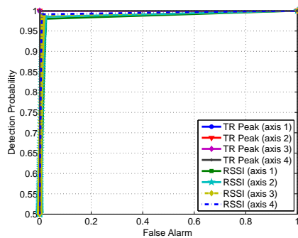
Fig. 14: ROC curve for distinguishing between S_1 and S_2 under LOC C.
