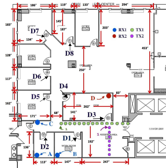
Fig. 5: Floorplan of the test environment.
