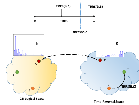
Fig. 3: Mapping between the CSI logical space and the time-reversal space.
