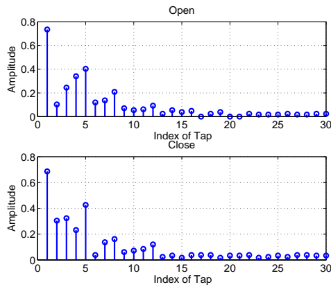
Fig. 9: Multipath profiles (amplitude part) of door D1 under LOC C.
