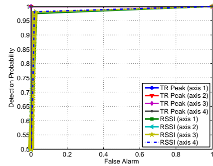
Fig. 15: ROC curve for distinguishing between S_1 and S_9 under LOC C.
