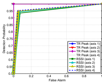
Fig. 11: ROC curve for distinguishing between S_1 and S_2 under LOC B.
