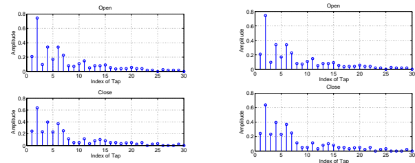
(a) Multipath profiles (amplitude part) when TX on location “1” (N-LOS). (b) Multipath profiles (amplitude part) when TX on location “5” (LOS).
