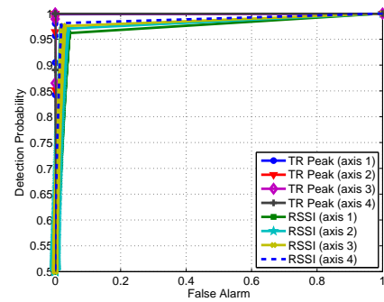
Fig. 12: ROC curve for distinguishing between S_1 and S_9 under LOC B.
