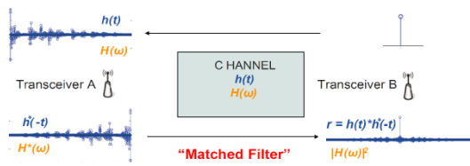
Fig. 2: TR-based wireless communication.
