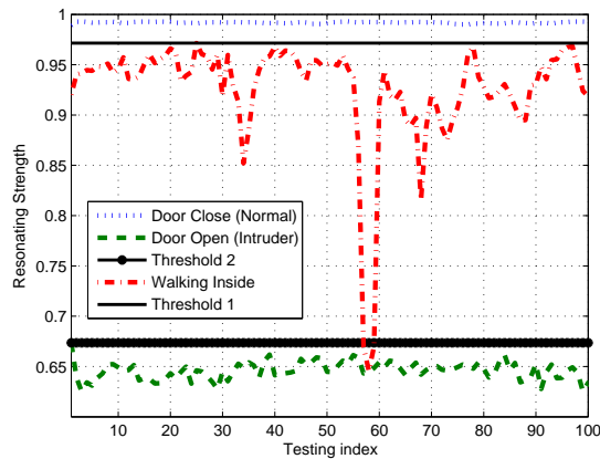
Fig. 18: Resonating strength of guard system.
