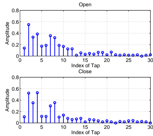
Fig. 7: Multipath profiles (amplitude part) of door D1 under LOC A.
